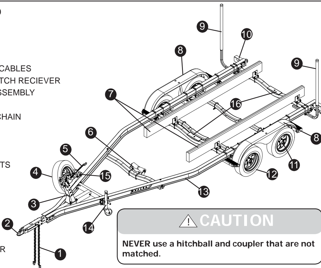
Bunk Trailer (Typical)
