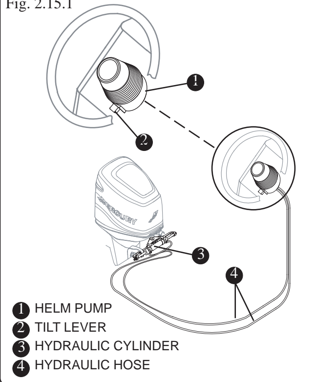
Hydraulic Tilt Steering Fig. 2.15.1
