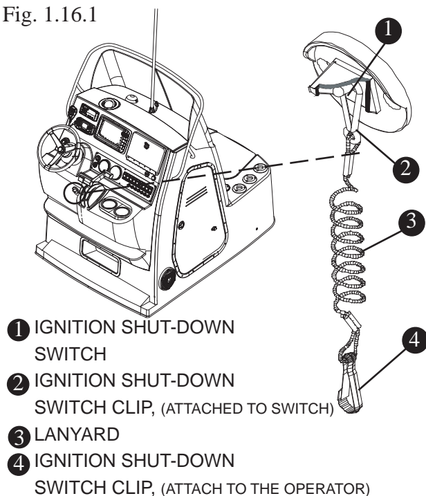
Emergency Engine Stop Switch
