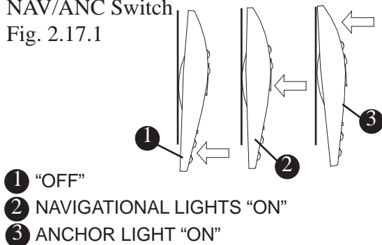
NAV/ANC Switch
