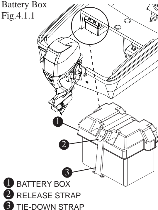
Battery Box
